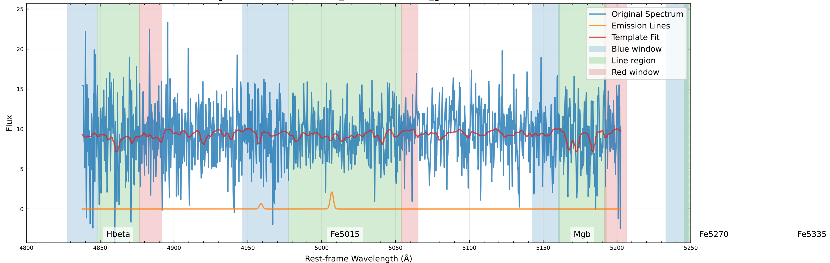
Original Data Comparison (v_star=81.6 km/s, v_gas=-44.7 km/s)
