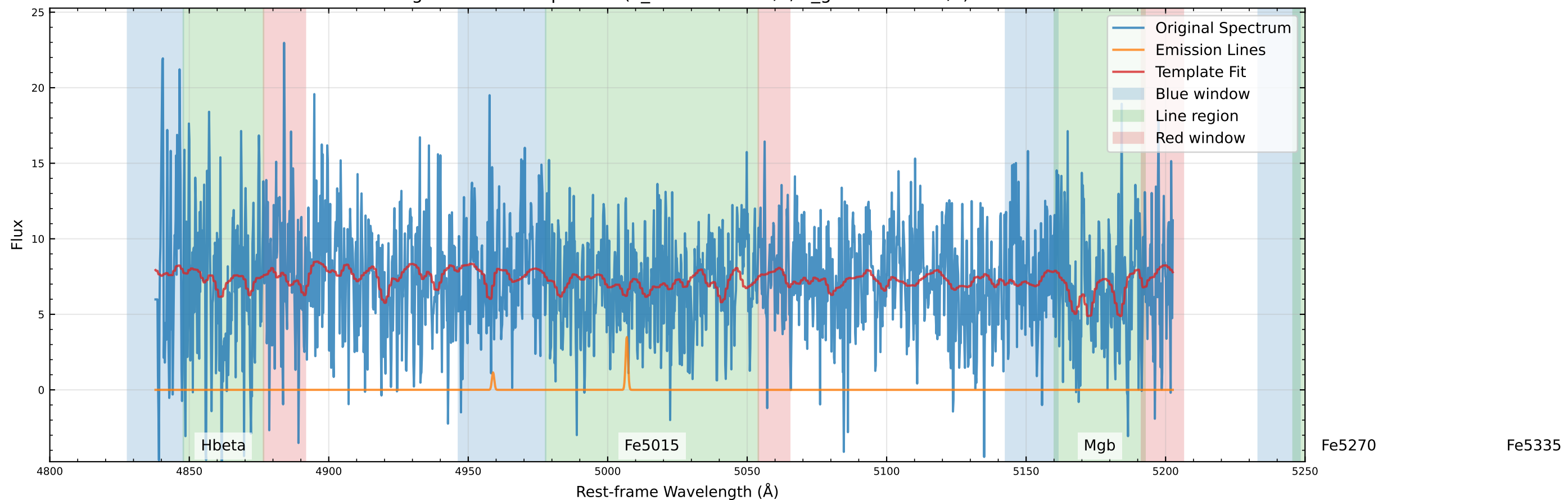
Original Data Comparison (v_star=85.1 km/s, v_gas=-21.6 km/s)
