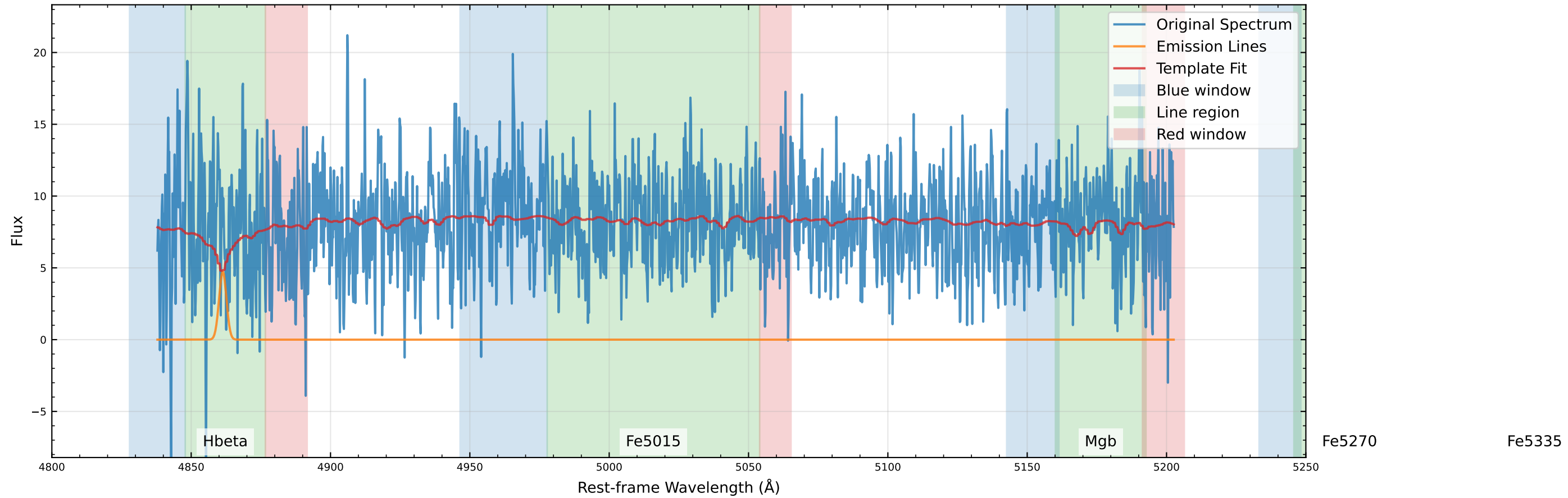
Original Data Comparison (v_star=-18.8 km/s, v_gas=-89.5 km/s)
