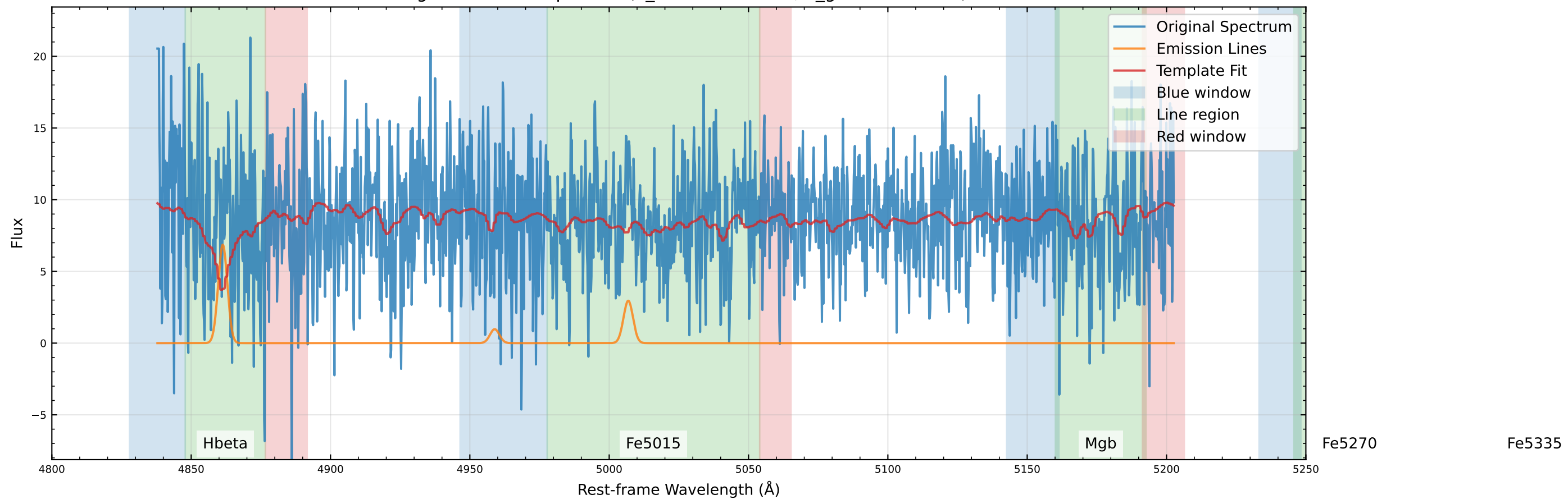
Original Data Comparison (v_star=56.1 km/s, v_gas=35.9 km/s)
