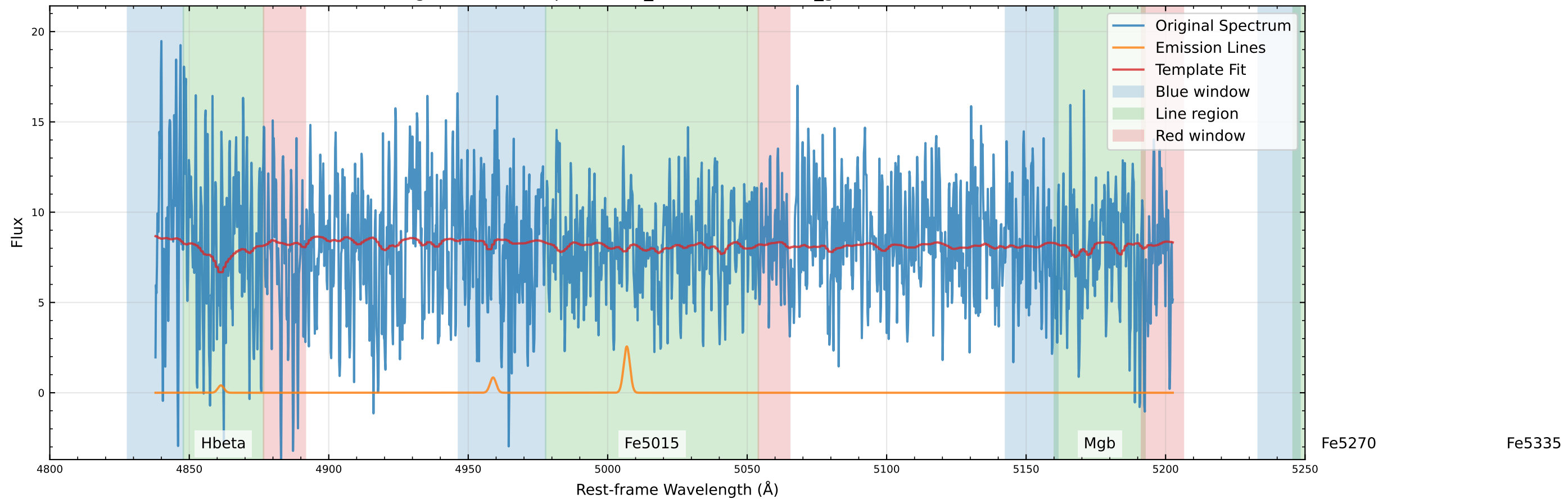
Original Data Comparison (v_star=13.4 km/s, v_gas=30.7 km/s)
