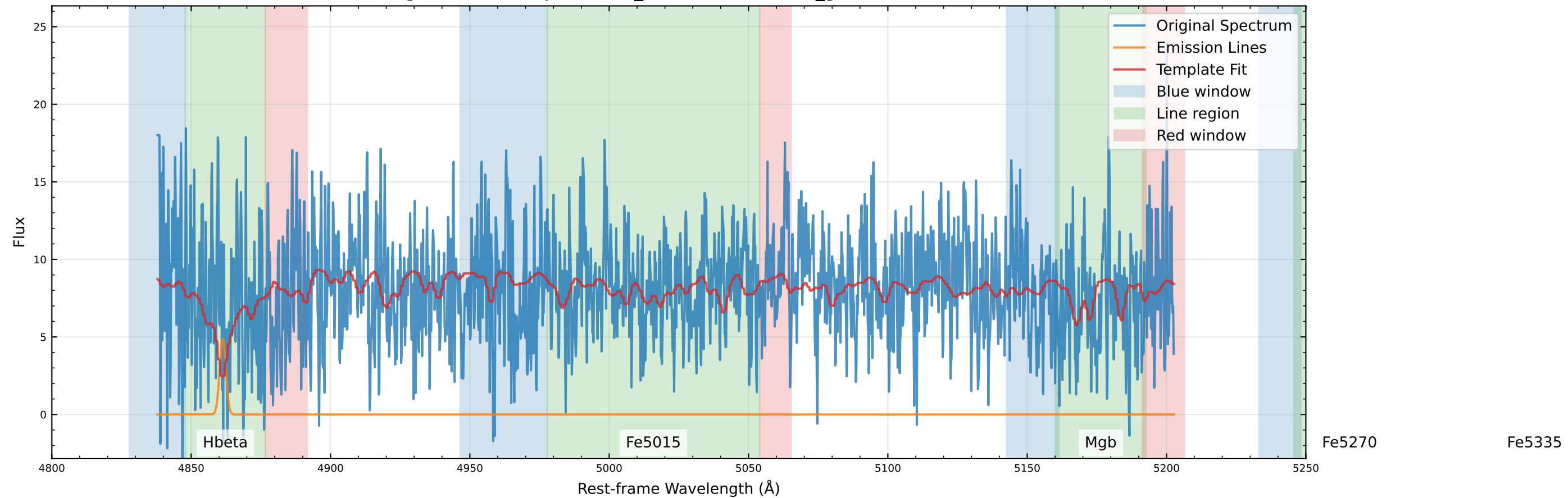
Original Data Comparison (v_star=183.8 km/s, v_gas=311.8 km/s)
