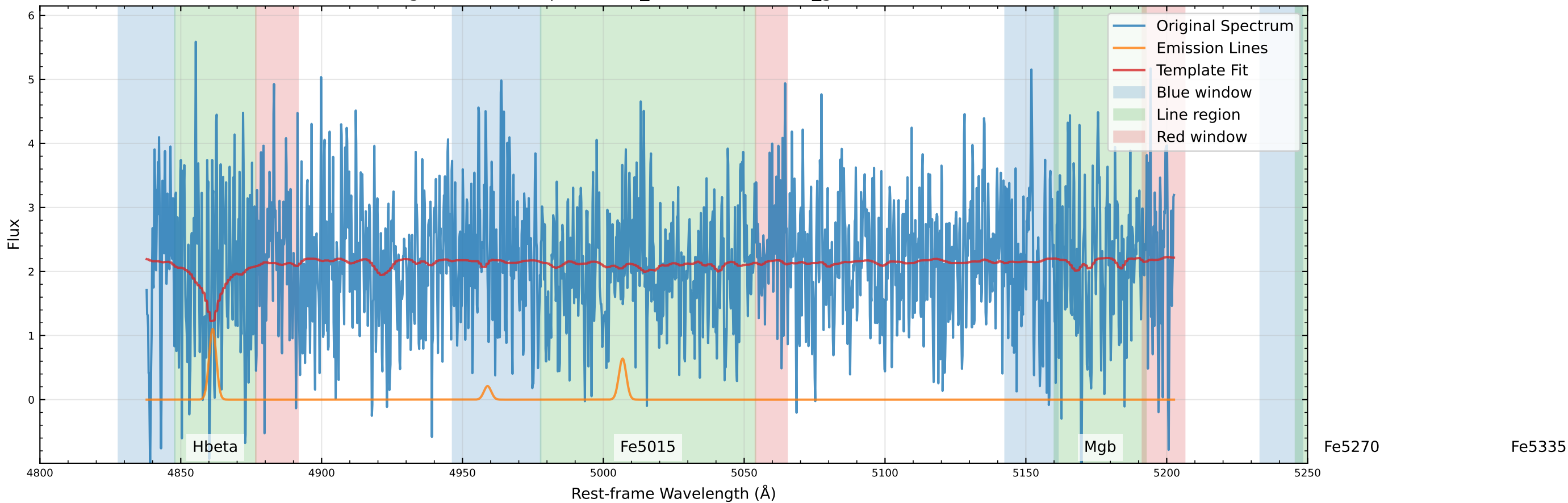
Original Data Comparison (v_star=50.9 km/s, v_gas=81.9 km/s)
