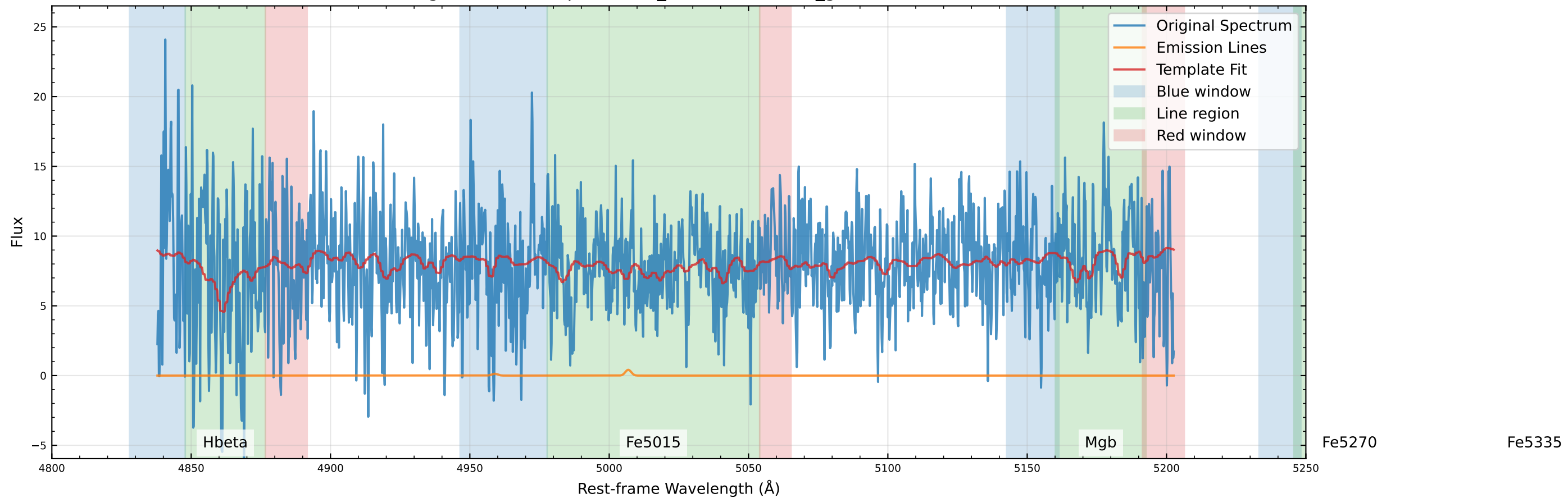
Original Data Comparison (v_star=2.8 km/s, v_gas=6.6 km/s)
