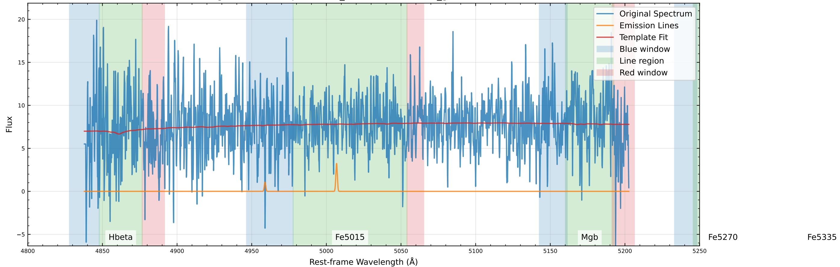
Original Data Comparison (v_star=120.8 km/s, v_gas=126.1 km/s)
