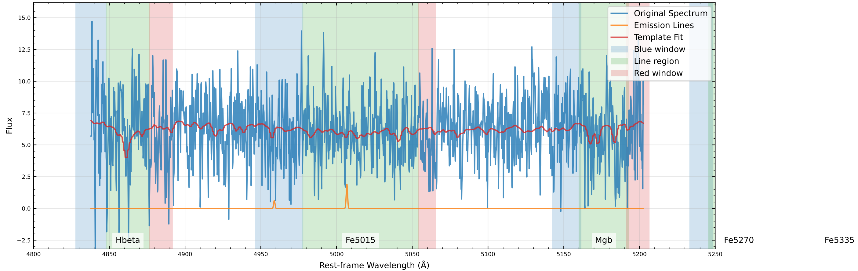
Original Data Comparison (v_star=72.1 km/s, v_gas=91.3 km/s)
