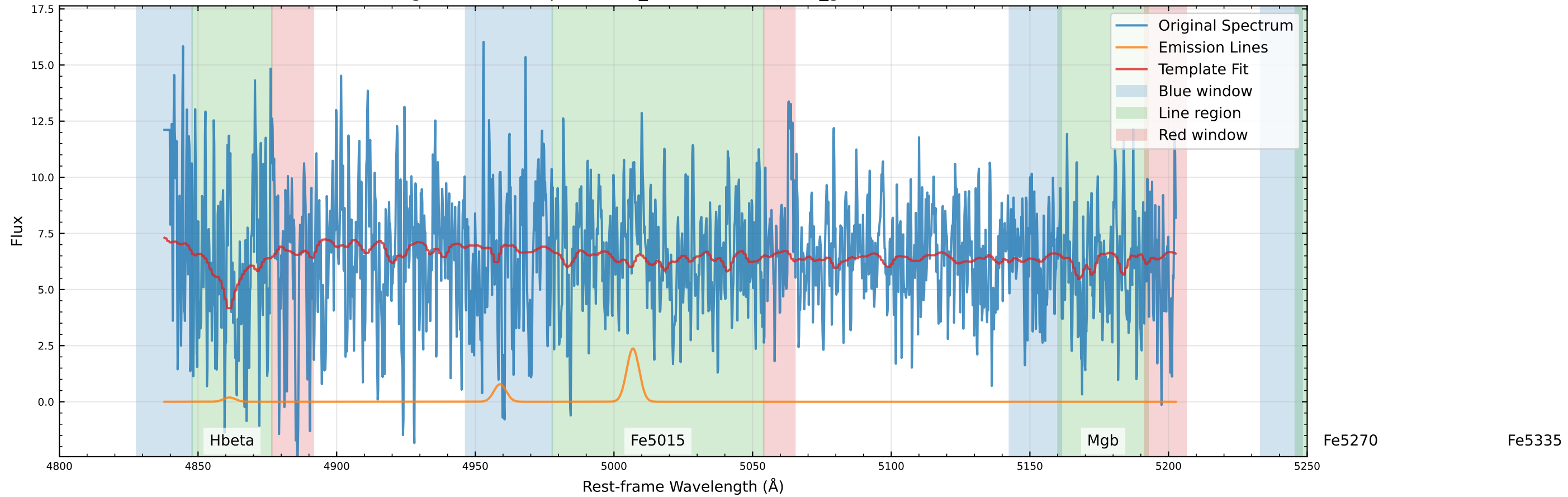
Original Data Comparison ( v_{\text{star}}=125.9 km/s, v_{\text{gas}}=101.3 km/s)
