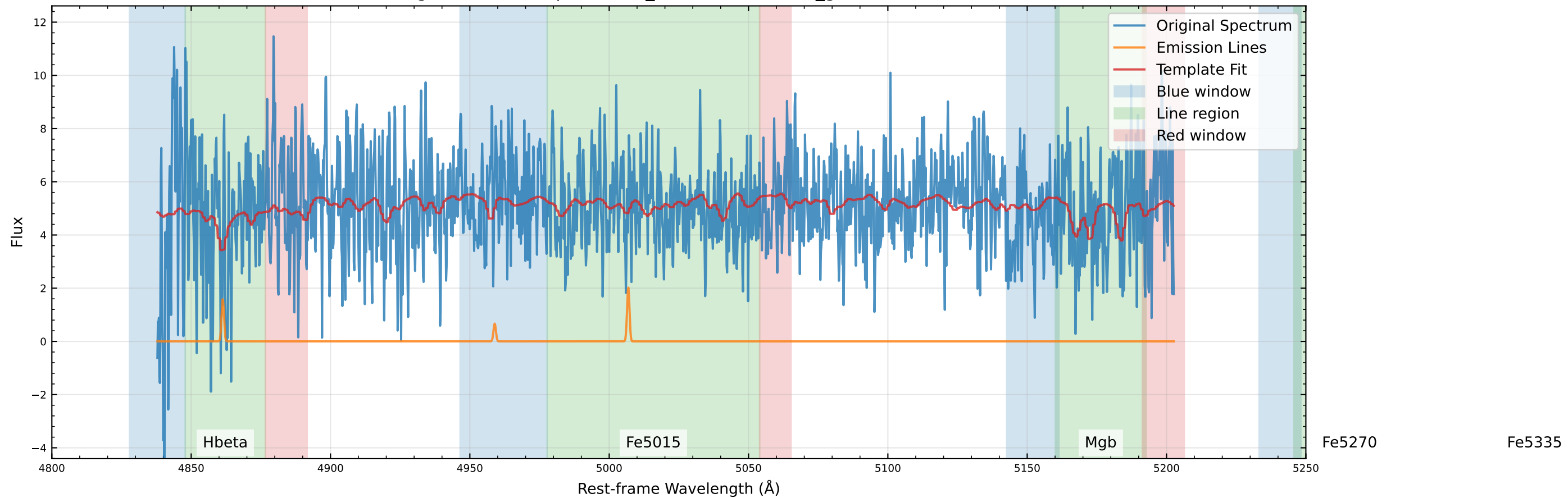
Original Data Comparison (v_star=20.3 km/s, v_gas=22.1 km/s)
