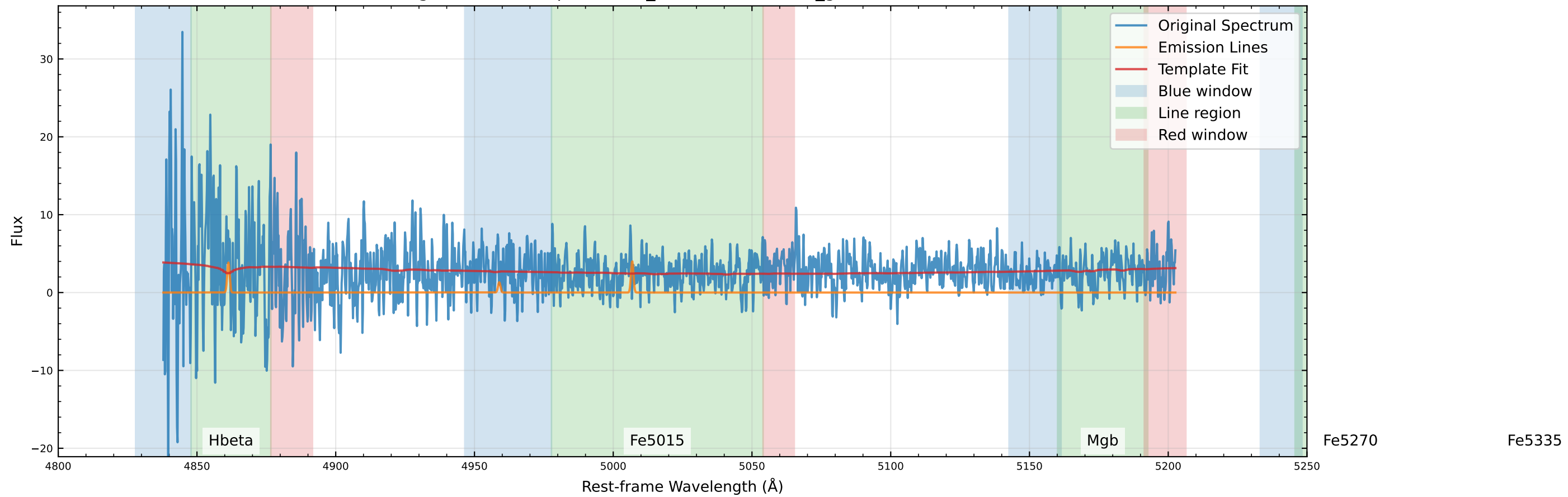
Original Data Comparison (v_star=23.1 km/s, v_gas=-35.6 km/s)
