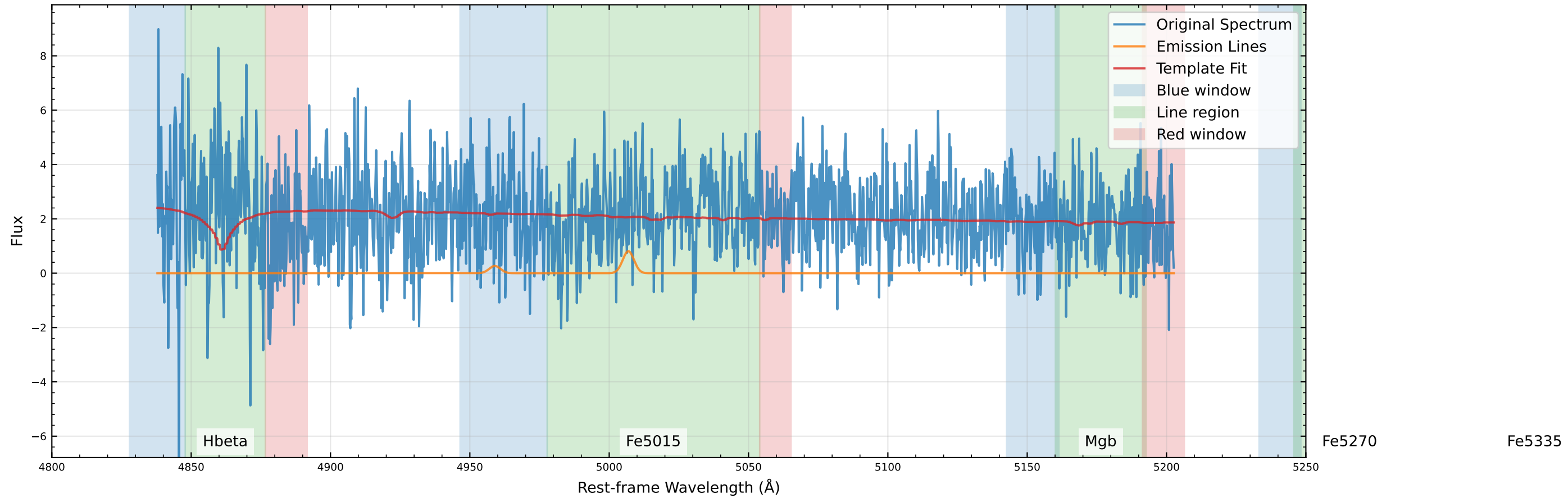
Original Data Comparison (v_star=888.2 km/s, v_gas=1041.7 km/s)
