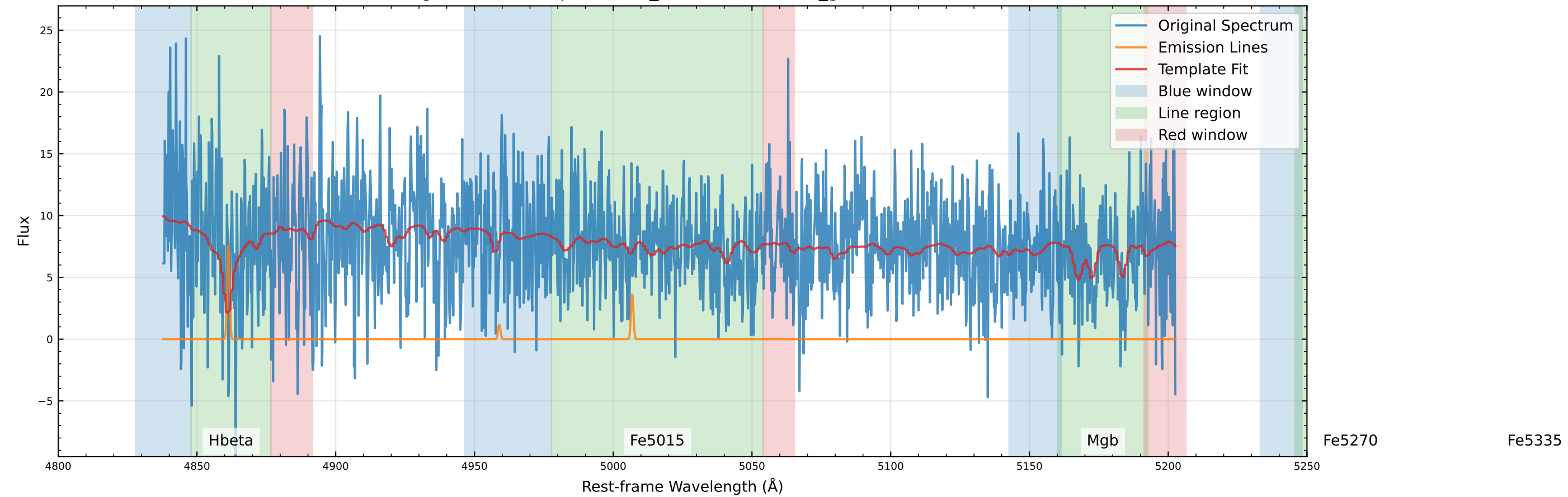
Original Data Comparison (v_star=46.2 km/s, v_gas=70.0 km/s)
