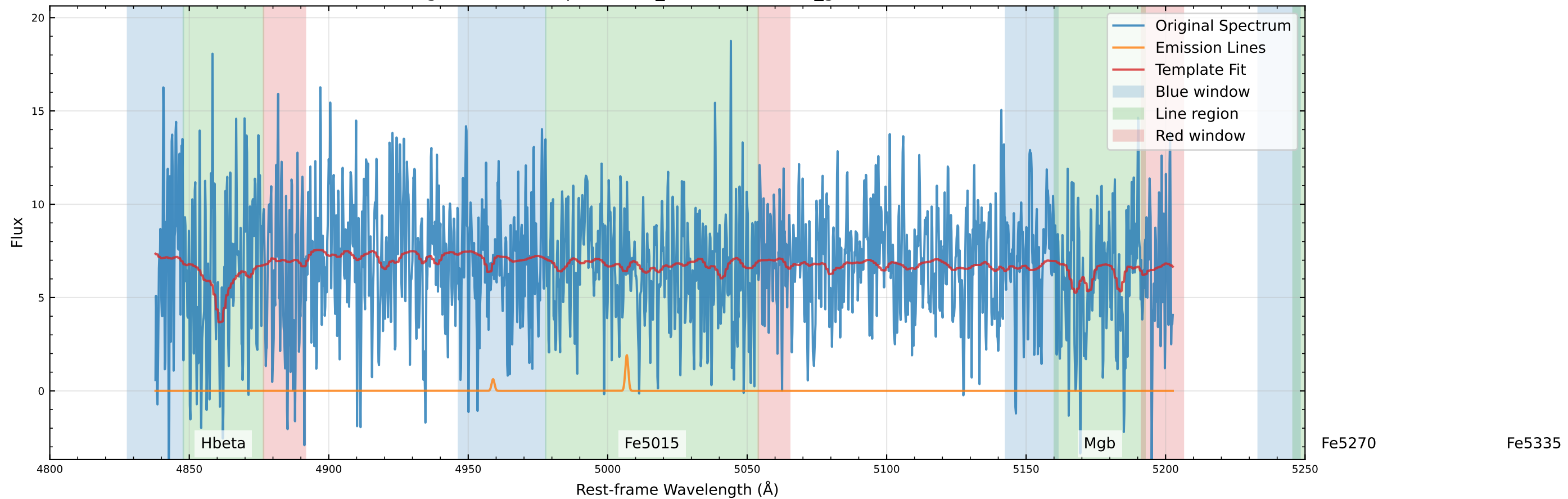
Original Data Comparison (v_star=0.3 km/s, v_gas=2.6 km/s)
