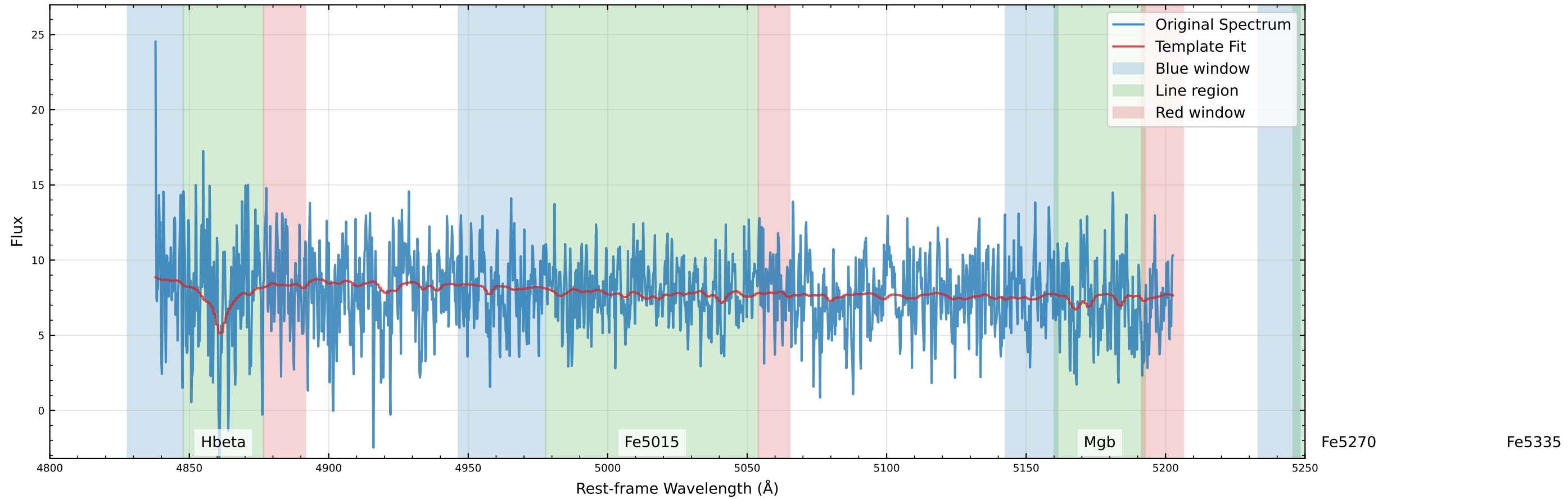
Original Data Comparison (v_star=-51.5 km/s)
