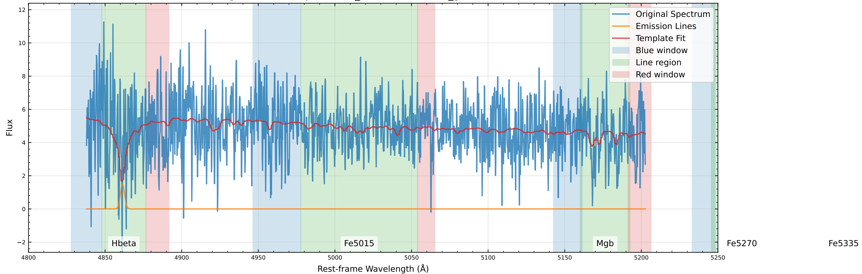
Original Data Comparison (v_star=13.9 km/s, v_gas=31.2 km/s)
