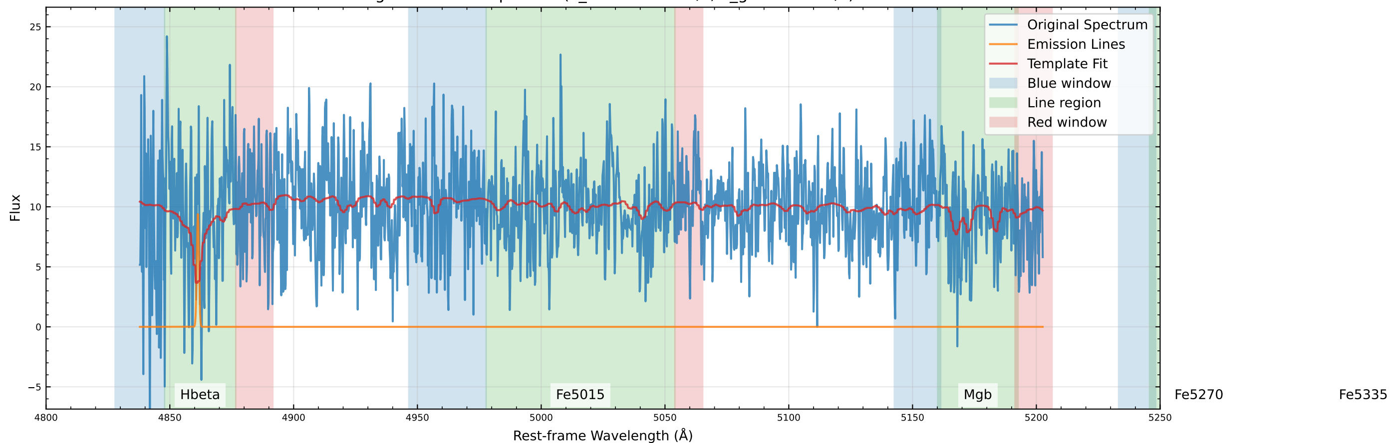
Original Data Comparison (v_star=35.7 km/s, v_gas=9.3 km/s)
