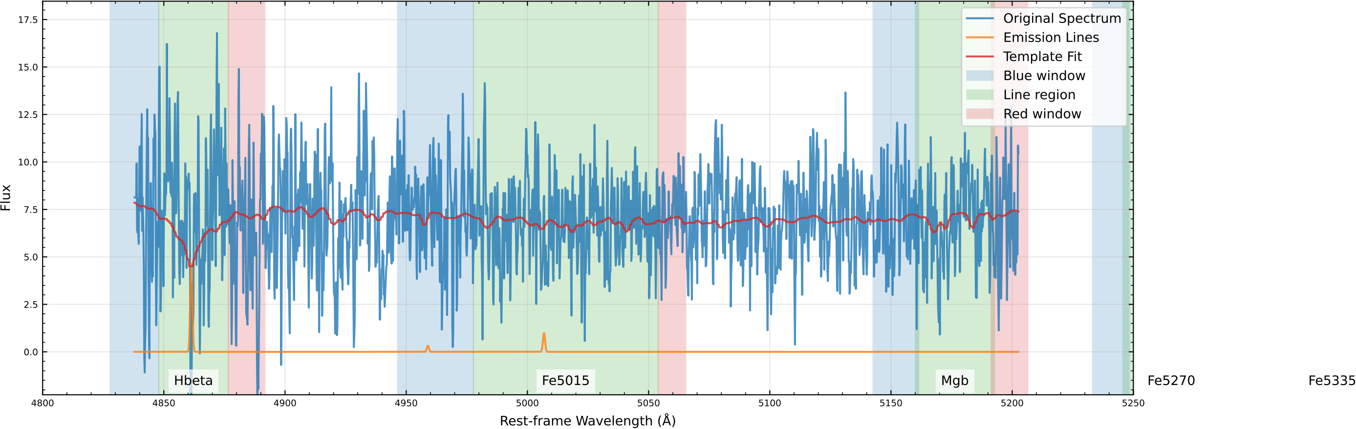
Original Data Comparison (v_star=120.7 km/s, v_gas=165.4 km/s)
