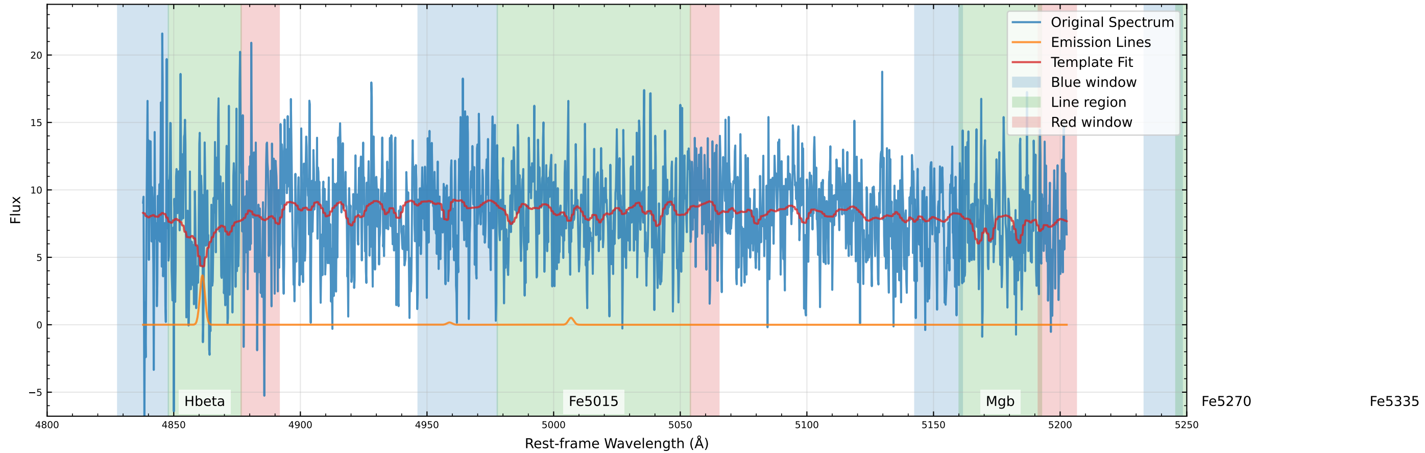
Original Data Comparison (v_star=-3.9 km/s, v_gas=-28.7 km/s)
