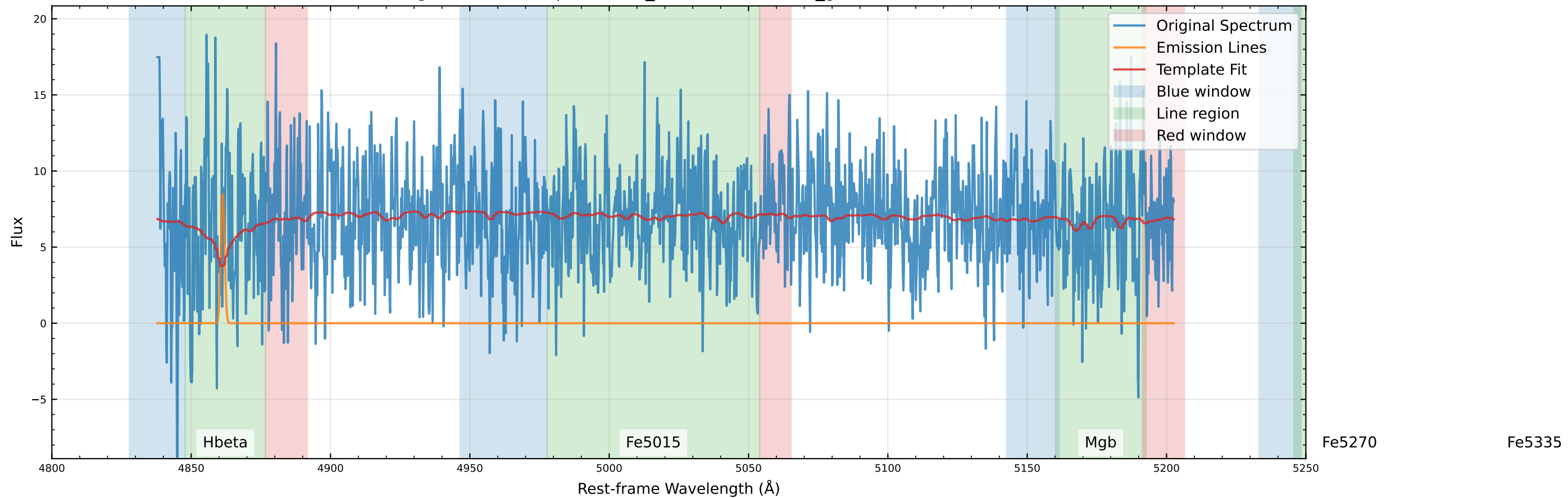
Original Data Comparison (v_star=68.7 km/s, v_gas=85.7 km/s)
