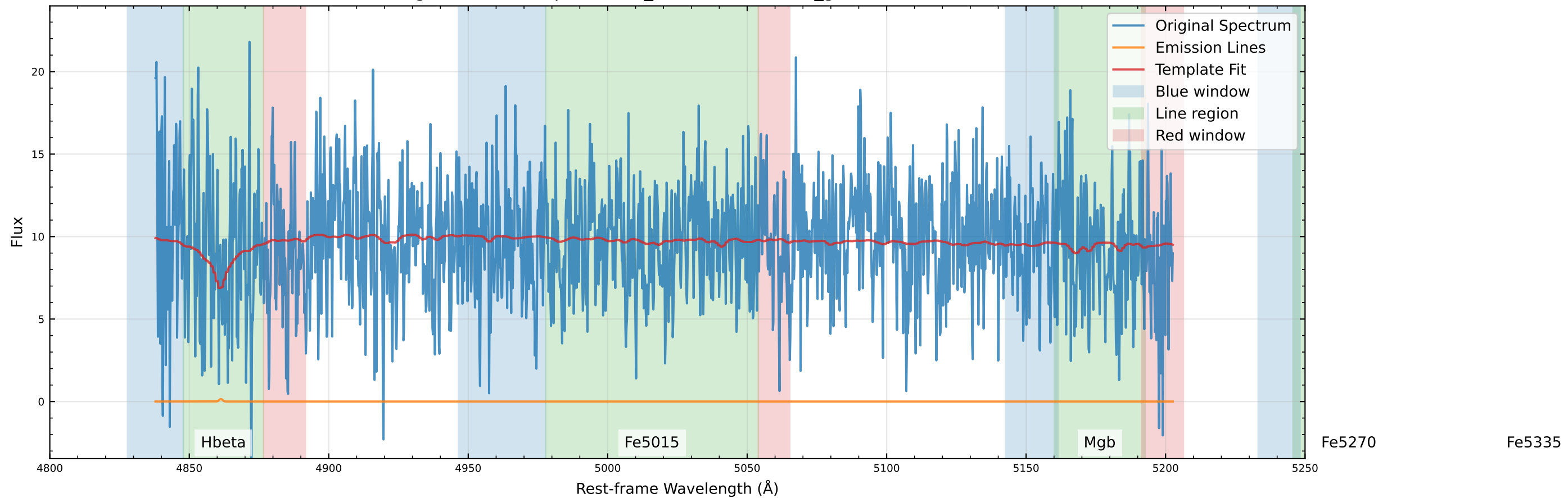
Original Data Comparison (v_star=25.0 km/s, v_gas=29.7 km/s)
