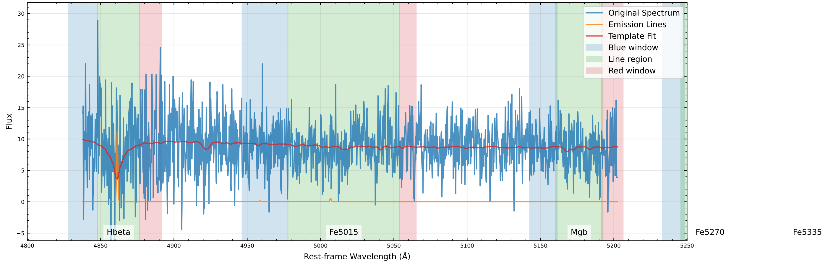
Original Data Comparison (v_star=-82.9 km/s, v_gas=-22.9 km/s)
