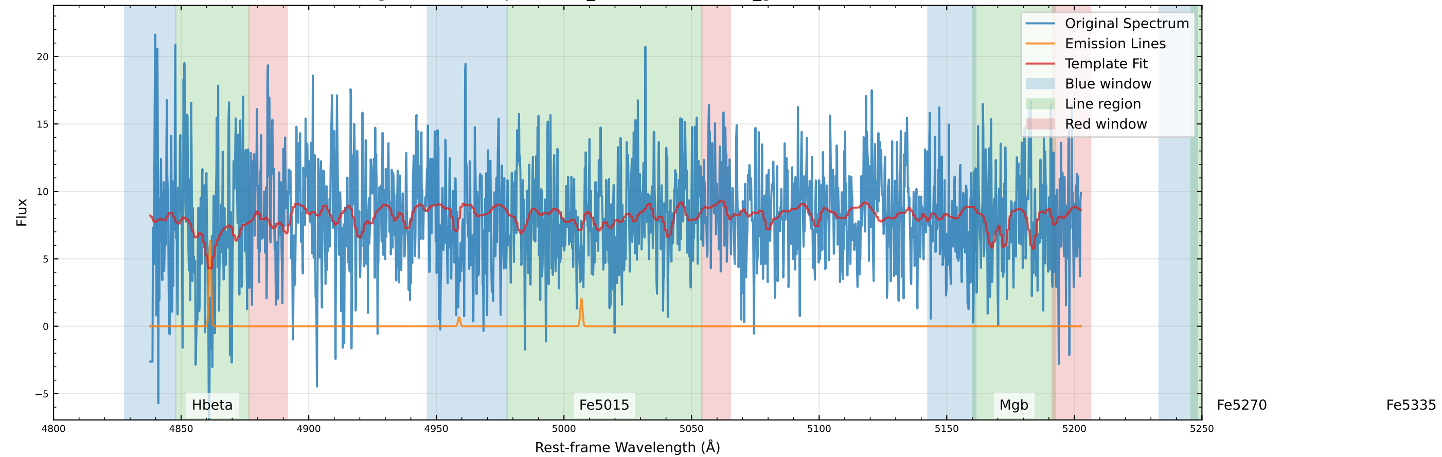
Original Data Comparison (v_star=128.9 km/s, v_gas=164.8 km/s)
