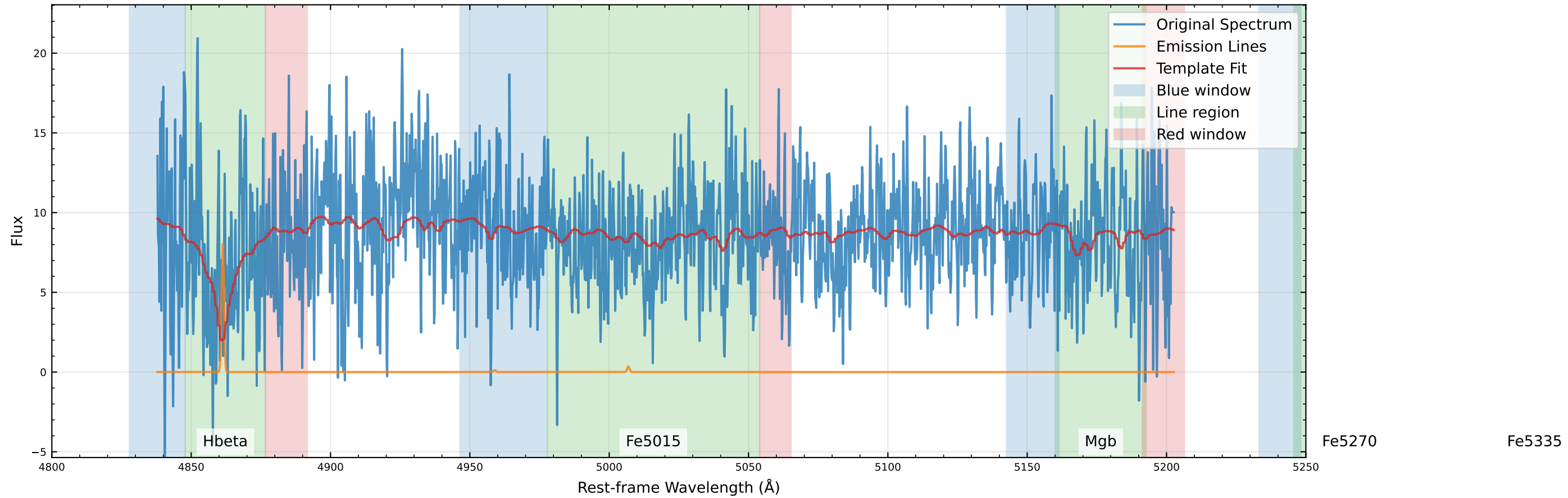
Original Data Comparison (v_star=-87.4 km/s, v_gas=-95.6 km/s)
