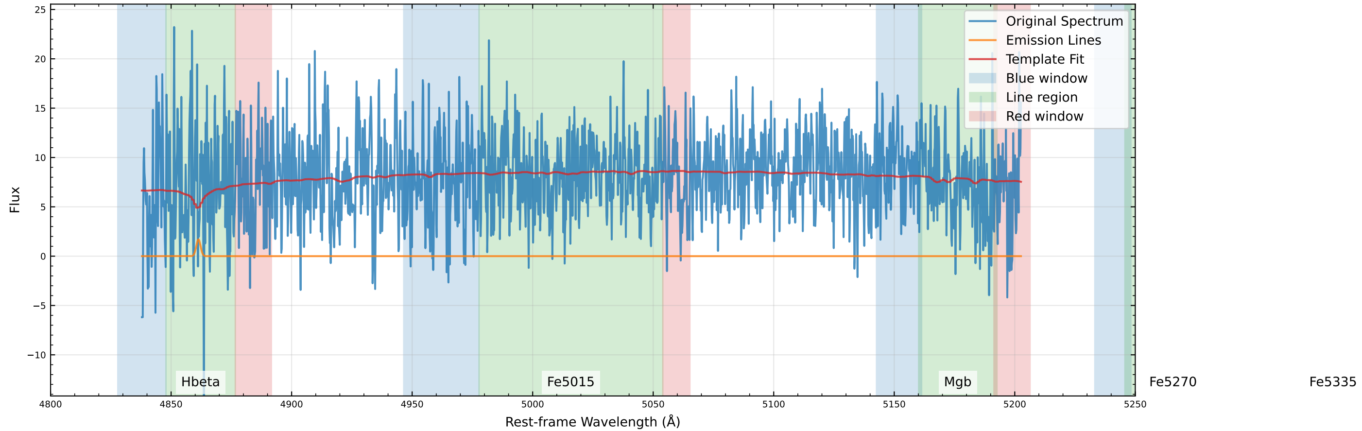
Original Data Comparison (v_star=46.9 km/s, v_gas=37.8 km/s)
