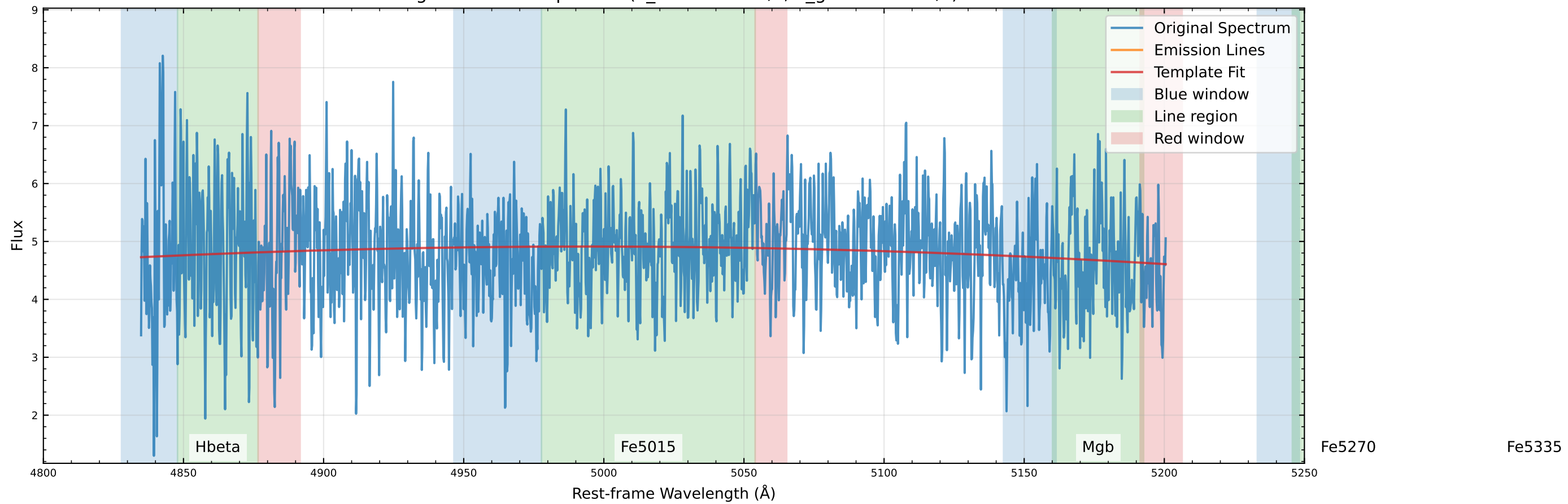
Original Data Comparison (v_star=0.0 km/s, v_gas=17.2 km/s)
