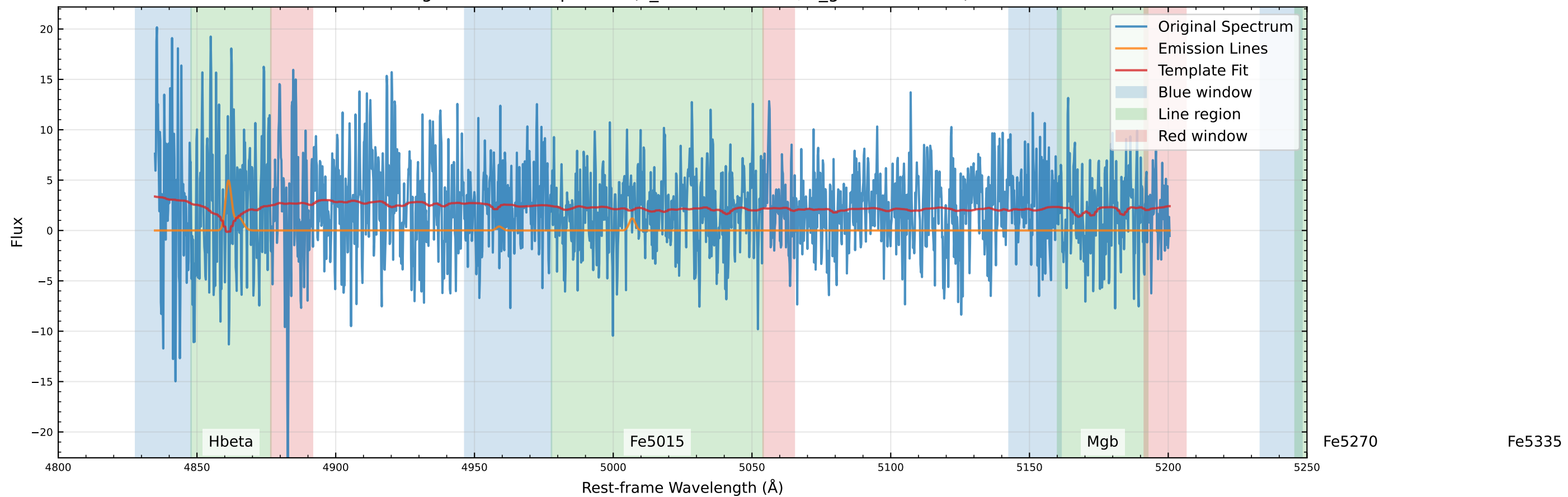
Original Data Comparison ( v_{\text{star}}=19.2 km/s, v_{\text{gas}}=88.5 km/s)
