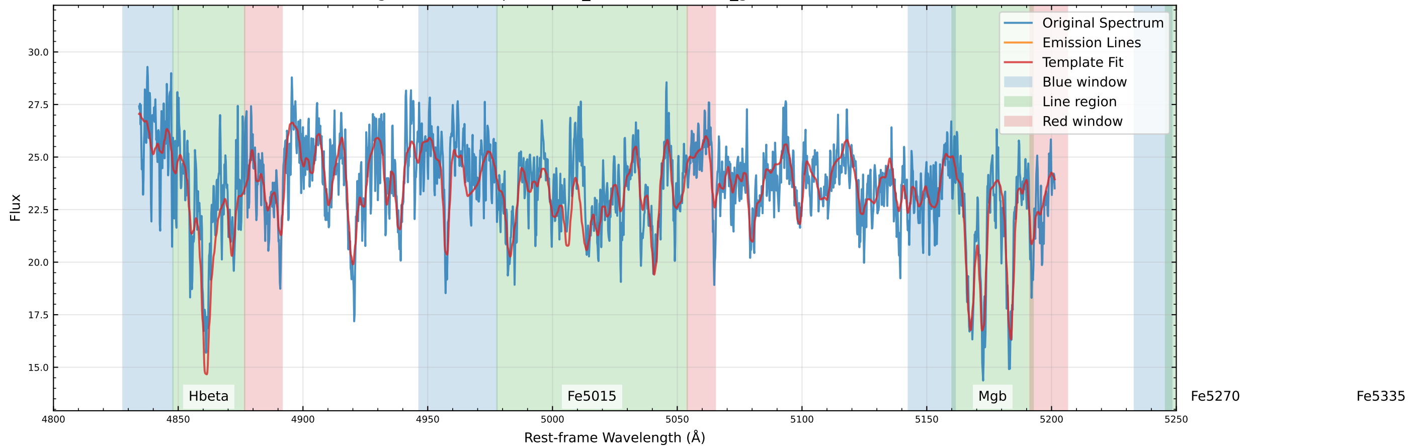
Original Data Comparison (v_star=-6.4 km/s, v_gas=119.5 km/s)
