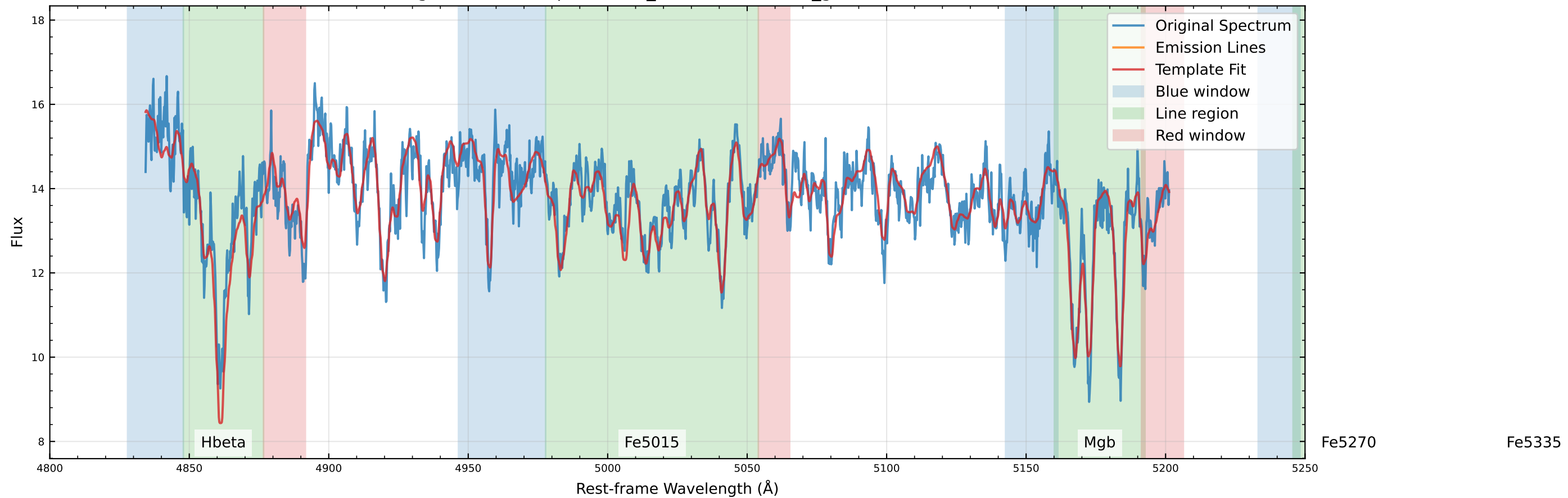
Original Data Comparison (v_star=-1.5 km/s, v_gas=32.9 km/s)
