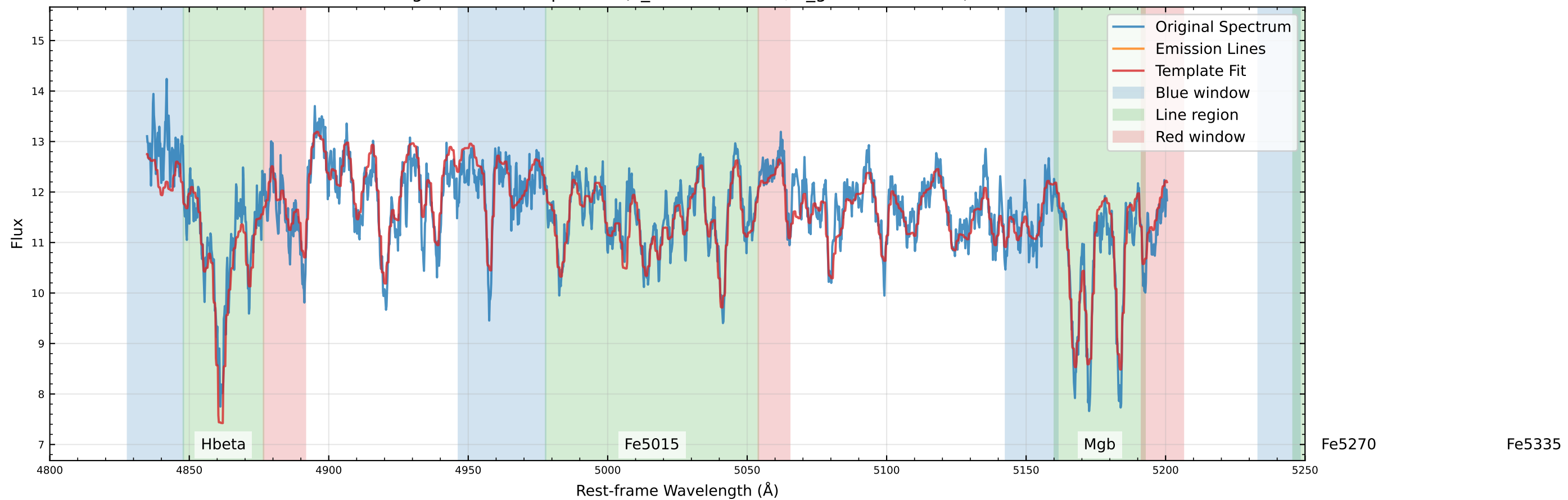
Original Data Comparison (v_star=-1.9 km/s, v_gas=187.1 km/s)
