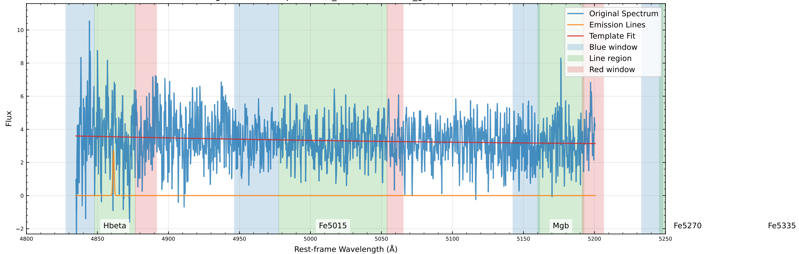
Original Data Comparison (v_star=0.0 km/s, v_gas=43.5 km/s)
