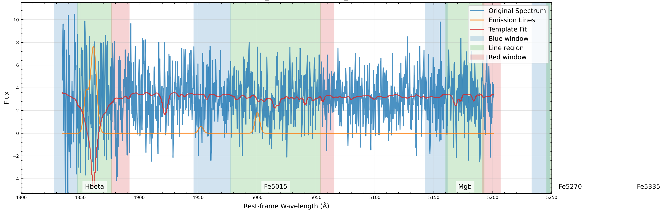
Original Data Comparison (v_star=-588.1 km/s, v_gas=-498.7 km/s)
