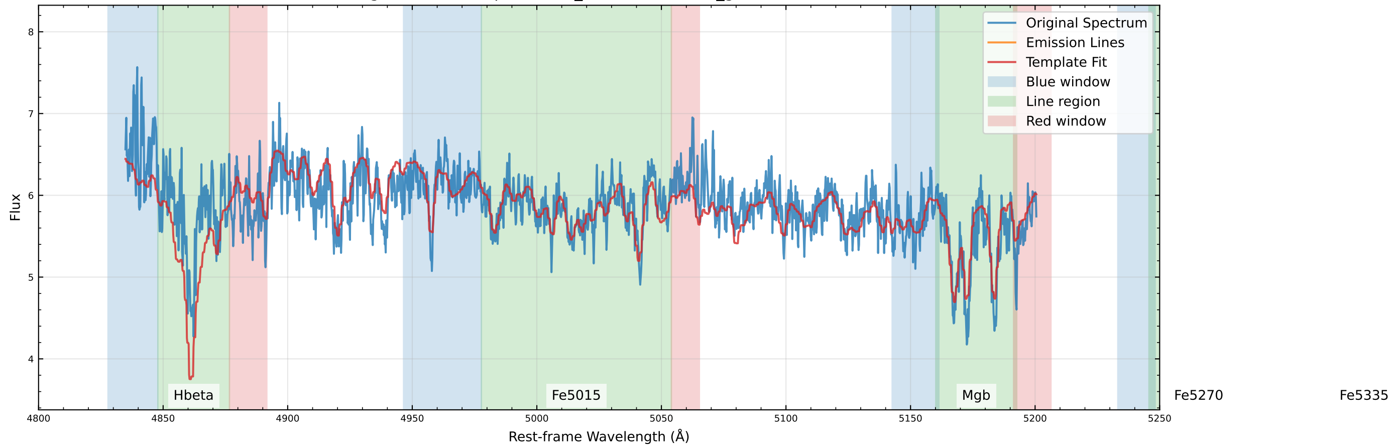
Original Data Comparison (v_star=7.9 km/s, v_gas=53.0 km/s)
