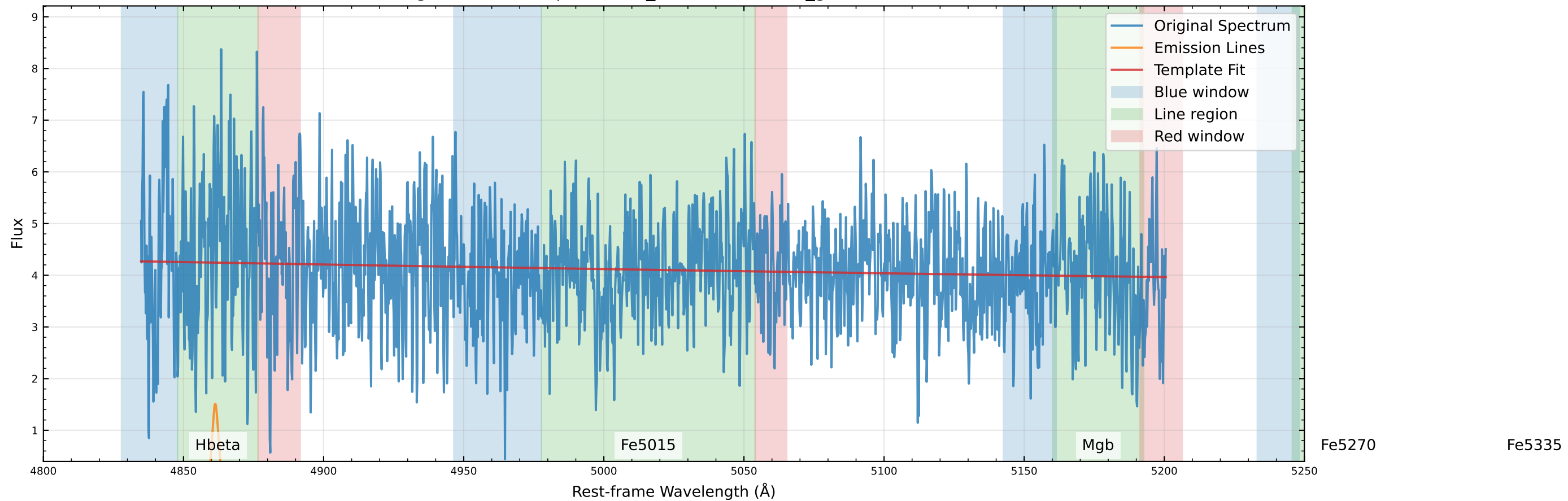
Original Data Comparison (v_star=0.0 km/s, v_gas=71.2 km/s)
