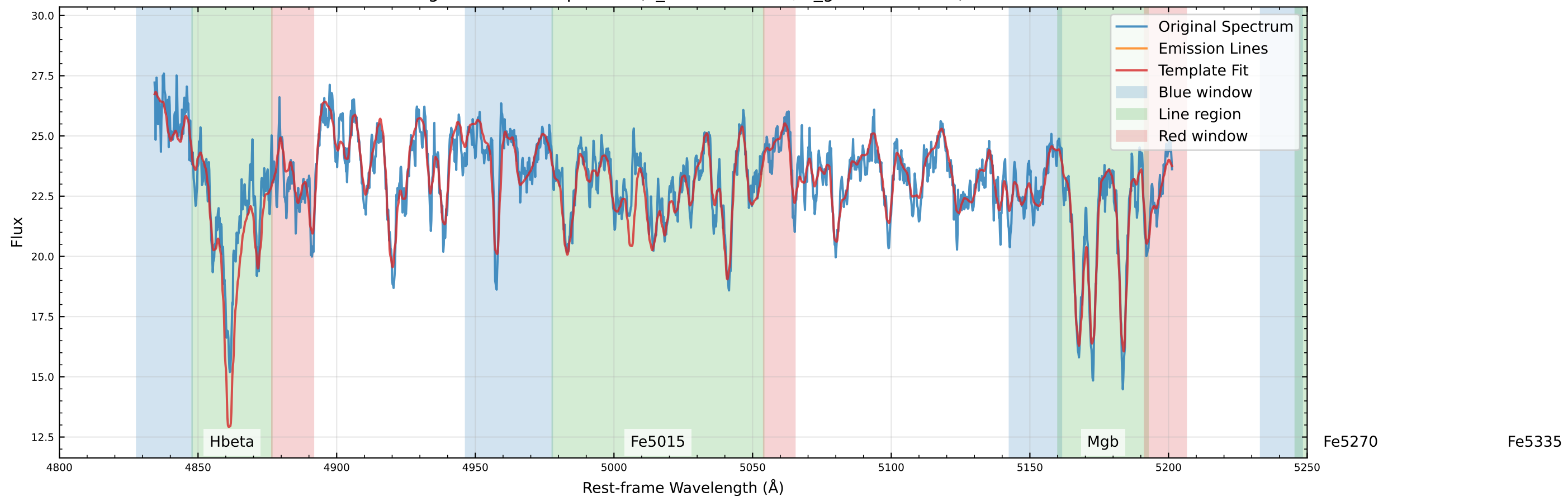
Original Data Comparison (v_star=1.8 km/s, v_gas=64.0 km/s)
