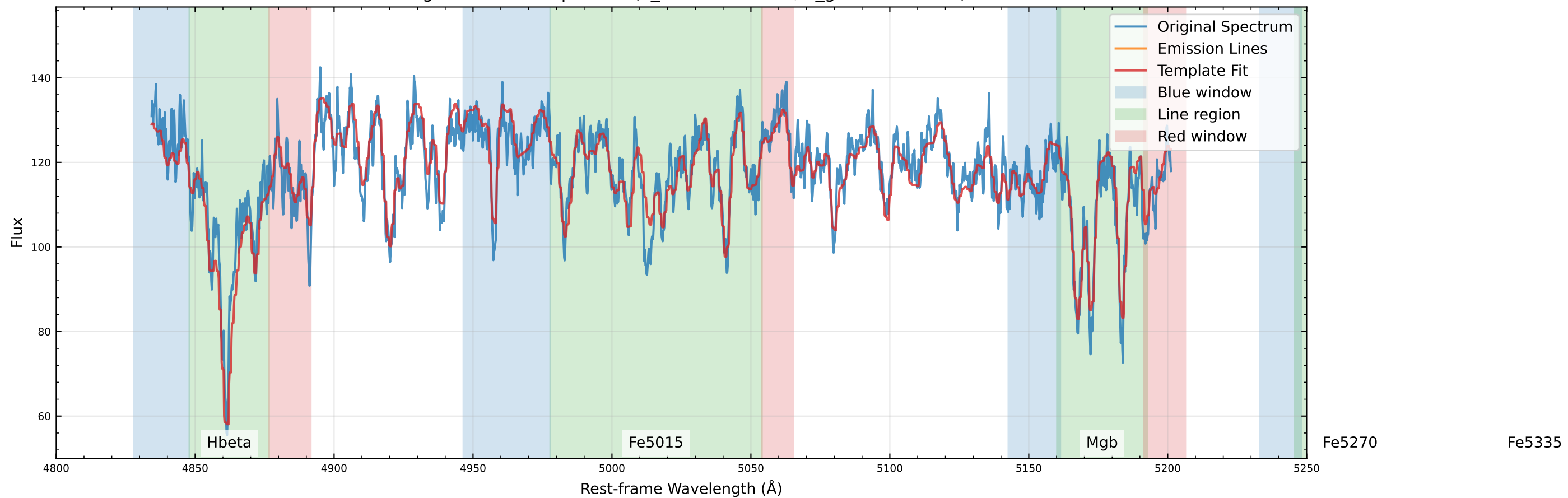
Original Data Comparison (v_star=-7.3 km/s, v_gas=34.8 km/s)
