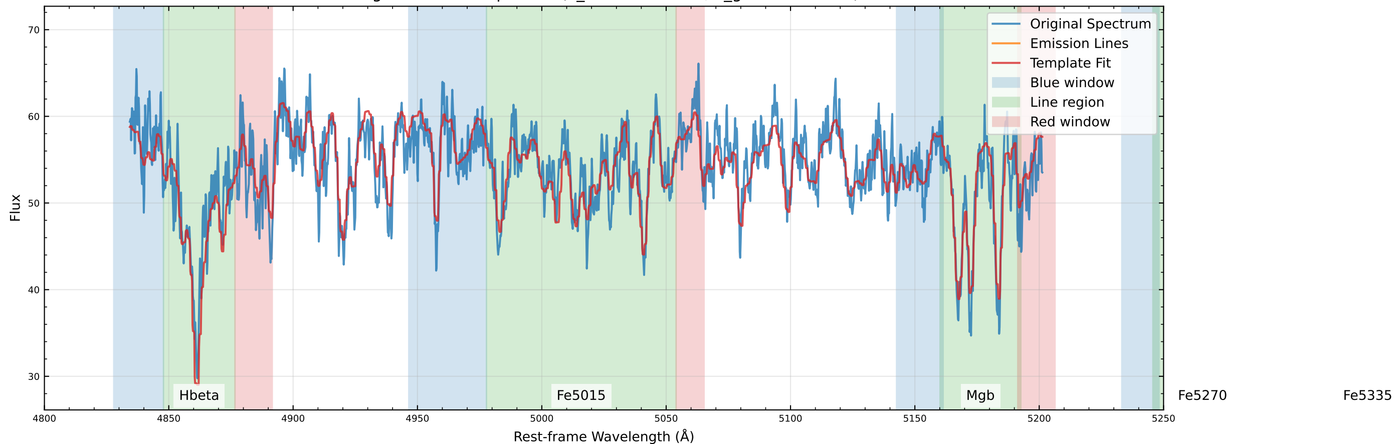
Original Data Comparison (v_star=-2.2 km/s, v_gas=49.8 km/s)
