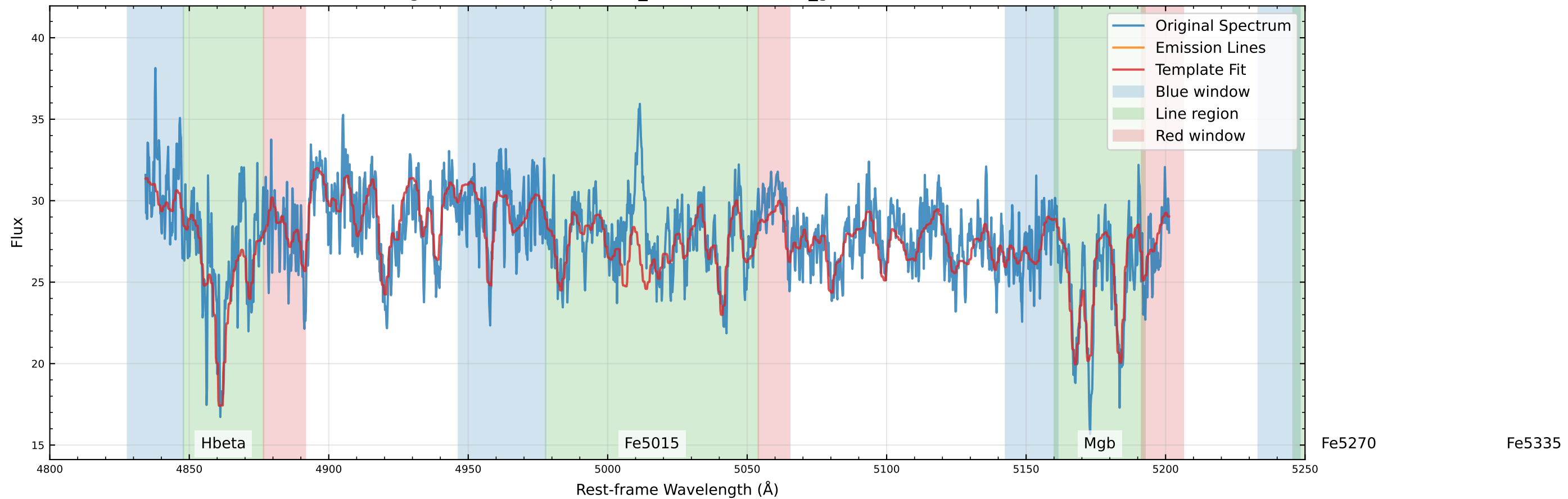
Original Data Comparison ( v_{\text{star}}=17.0 km/s, v_{\text{gas}}=244.8 km/s)
