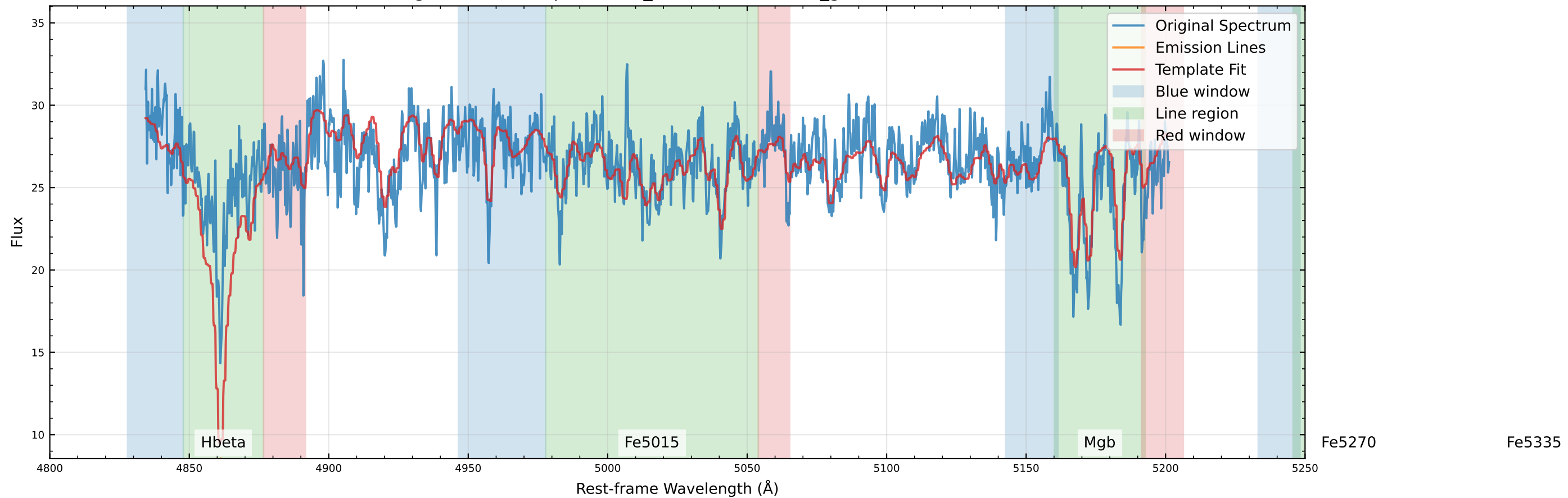
Original Data Comparison (v_star=-21.4 km/s, v_gas=-7.0 km/s)
