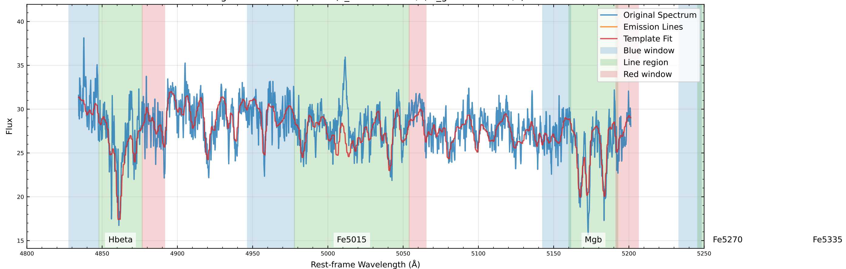
Original Data Comparison (v_star=17.0 km/s, v_gas=244.8 km/s)
