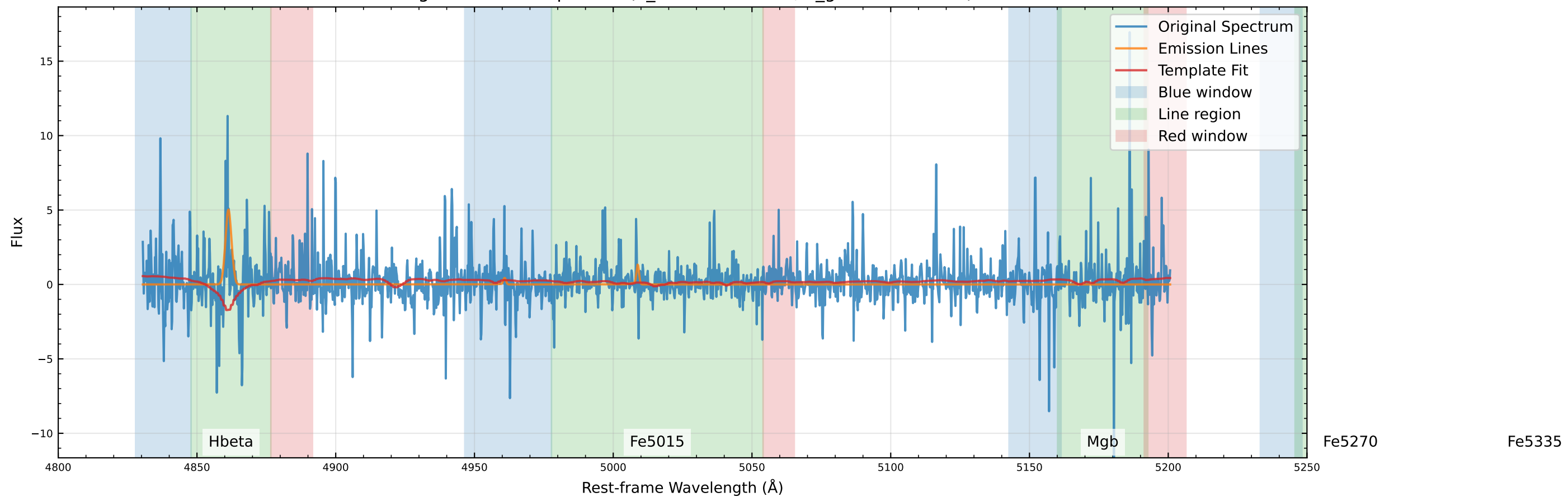
Original Data Comparison (v_star=78.2 km/s, v_gas=-30.4 km/s)
