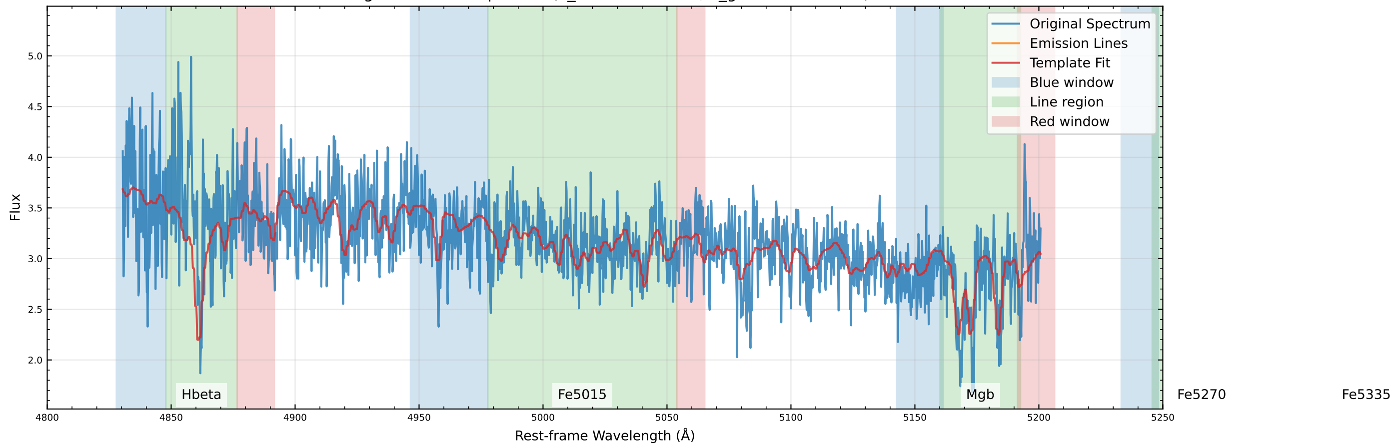
Original Data Comparison (v_star=27.1 km/s, v_gas=-163.6 km/s)
