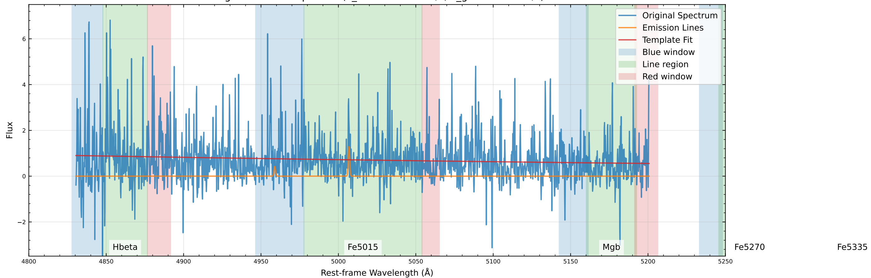
Original Data Comparison (v_star=-124.1 km/s, v_gas=-15.5 km/s)
