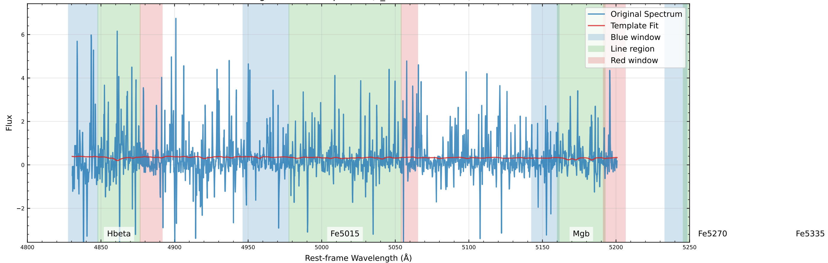
Original Data Comparison ( v_{\text{star}}=-221.8 km/s)
