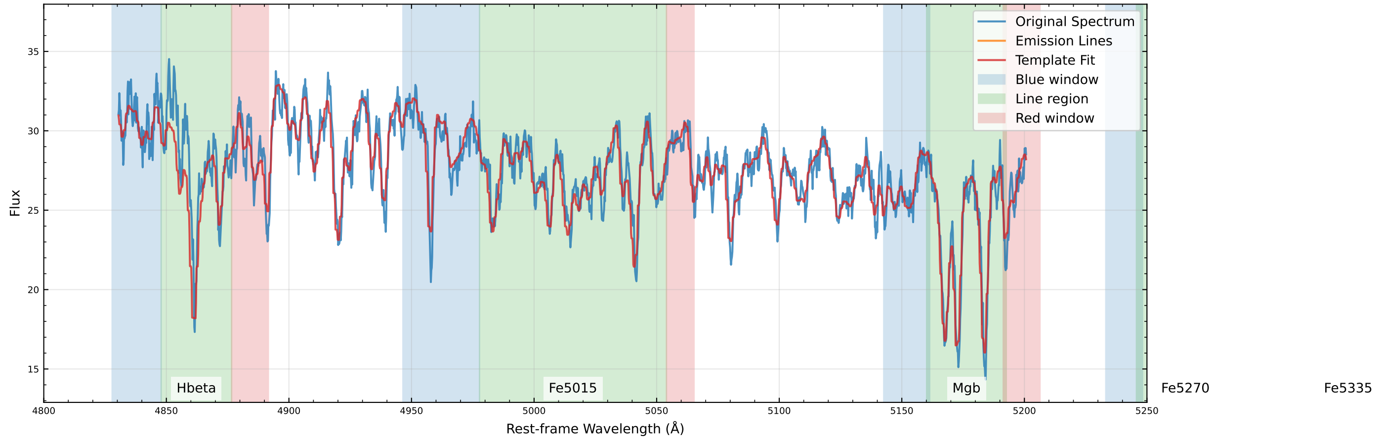
Original Data Comparison (v_star=20.0 km/s, v_gas=-280.0 km/s)
