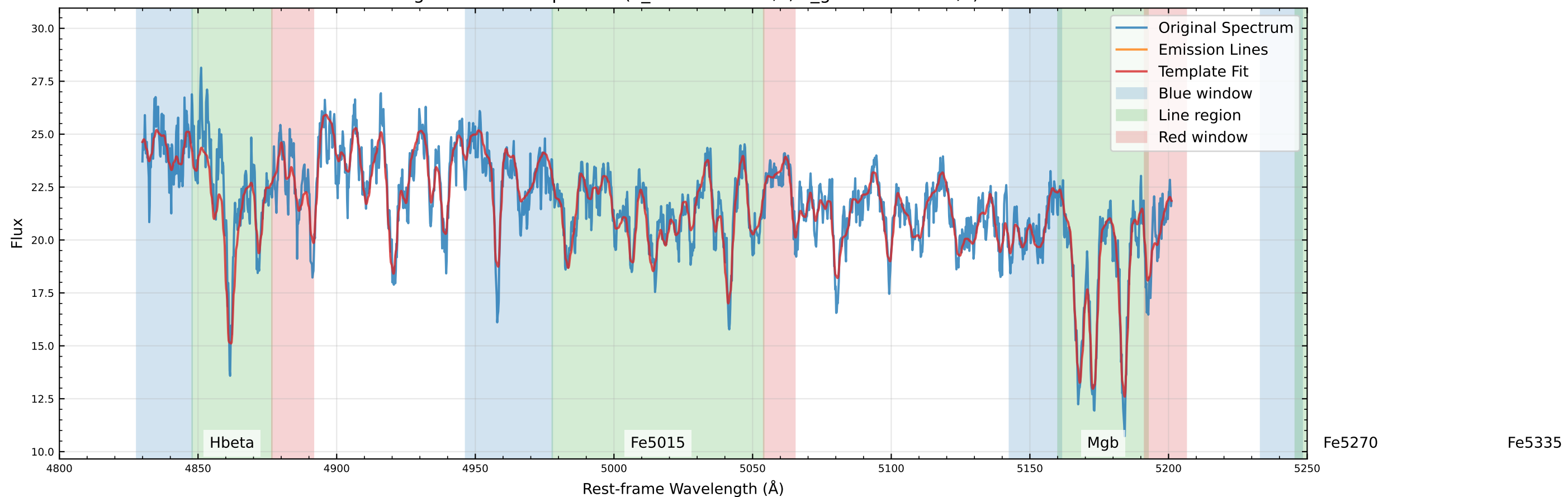
Original Data Comparison (v_star=20.7 km/s, v_gas=-204.8 km/s)
