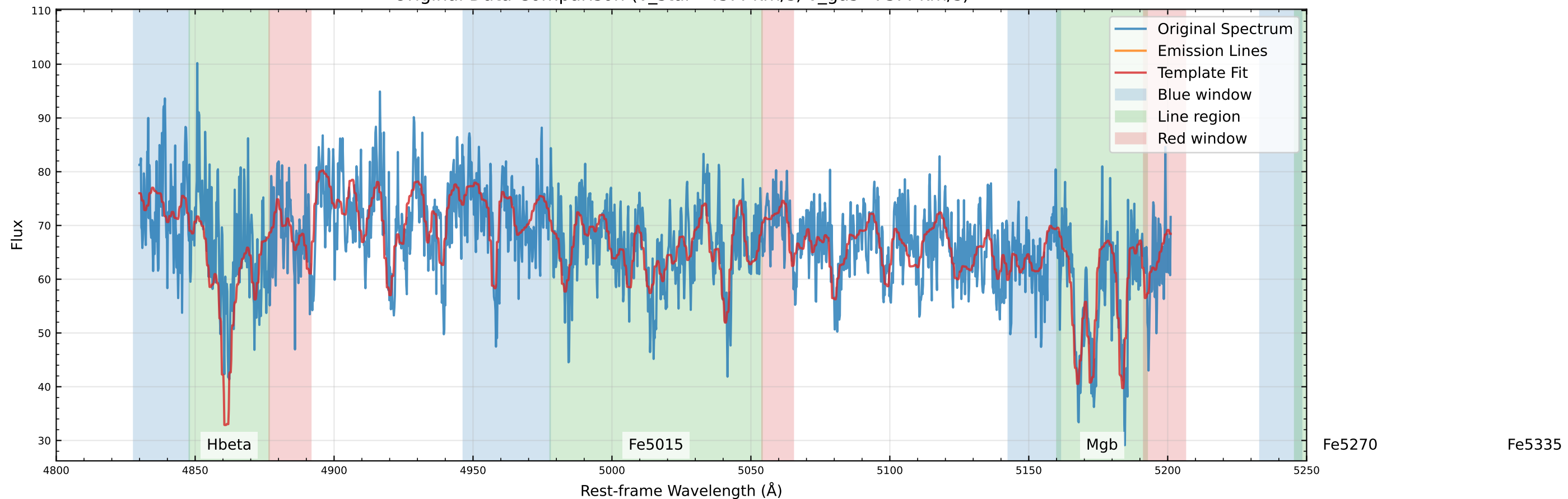
Original Data Comparison (v_star=45.4 km/s, v_gas=73.4 km/s)
