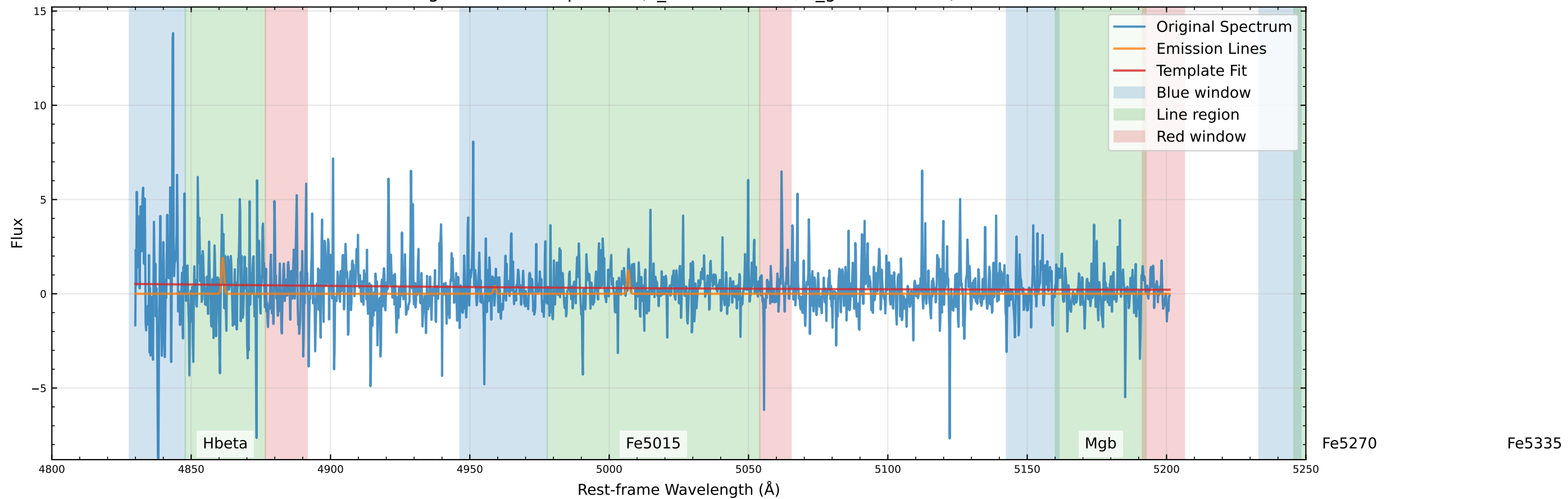
Original Data Comparison (v_star=0.0 km/s, v_gas=1.1 km/s)
